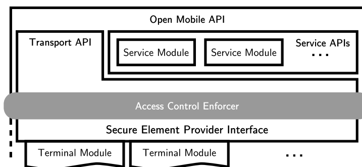
Fig. 3. Architecture of the Open Mobile API [11]
